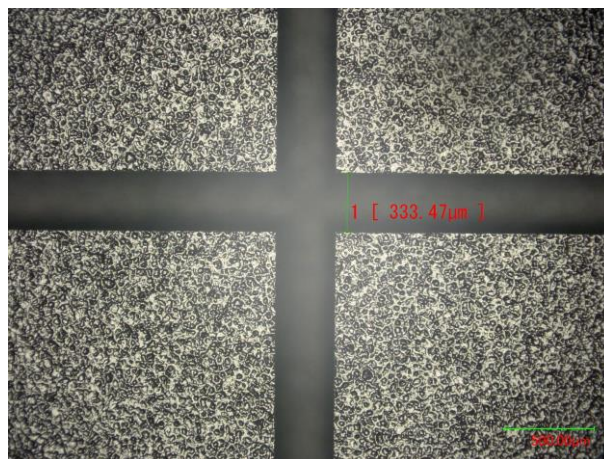
PICTURE 1: Microscope image of Mold compound (bright field illumination; top view)
